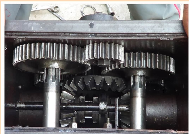
Transmission Train
